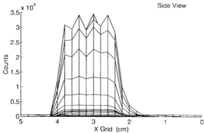
Figure 4.16. End and side views of the monostatic acoustic pulse for 1.3 MHz and wire of radius 64 microns.
